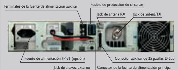
PANEL TRASERO
